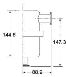
DN25KF
