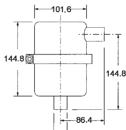
1" tube connection
