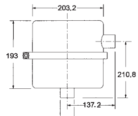
1 1/2" tube connection
