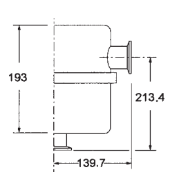
DN40KF/DN50KF
