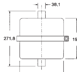
1 1/2" tube connection
