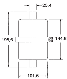
1" tube connection
